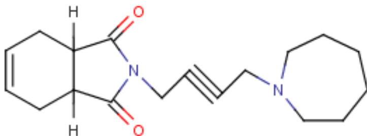
AM-3: 2-[4-(azepan-1-yl)but-2-yn-1-yl]-2,3,3a,4,7,7a-hexahydro-1H-isoindole-1,3-dione
