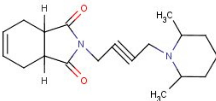
AM-2: 2-[4-(2,6-dimethylpiperidin-1-yl)but-2-yn-1-yl]-2,3,3a,4,7,7a-hexahydro-1H-isoindole-1,3-dione
