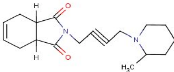
AM-1: 2-[4-(2-methylpiperidin-1-yl)but-2-yn-1-yl]-2,3,3a,4,7,7a-hexahydro-1H-isoindole-1,3-dione
